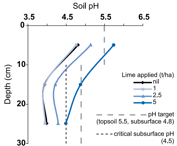
Figure 22 Soil pH measured 17 years after the initial lime application
